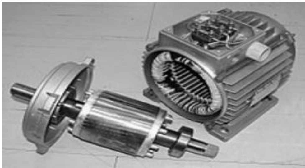
Fig Q1c : 4 poles, 36 slots, three phase induction motor (10 marks)
