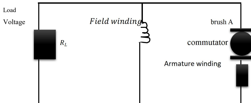
Fig. Q1d: Shunt wound D.C generator (5 marks)
